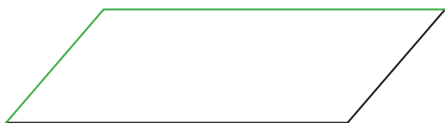
parallellogram
